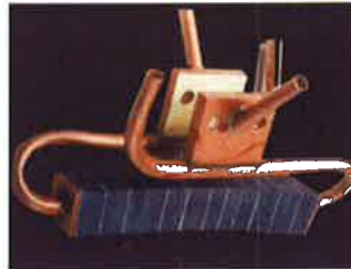
Single Turn Seam Anneal Coils
